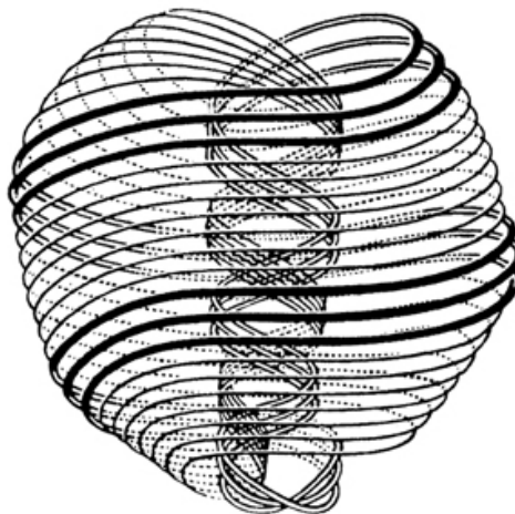
Figure 1 – Subatomic particle
